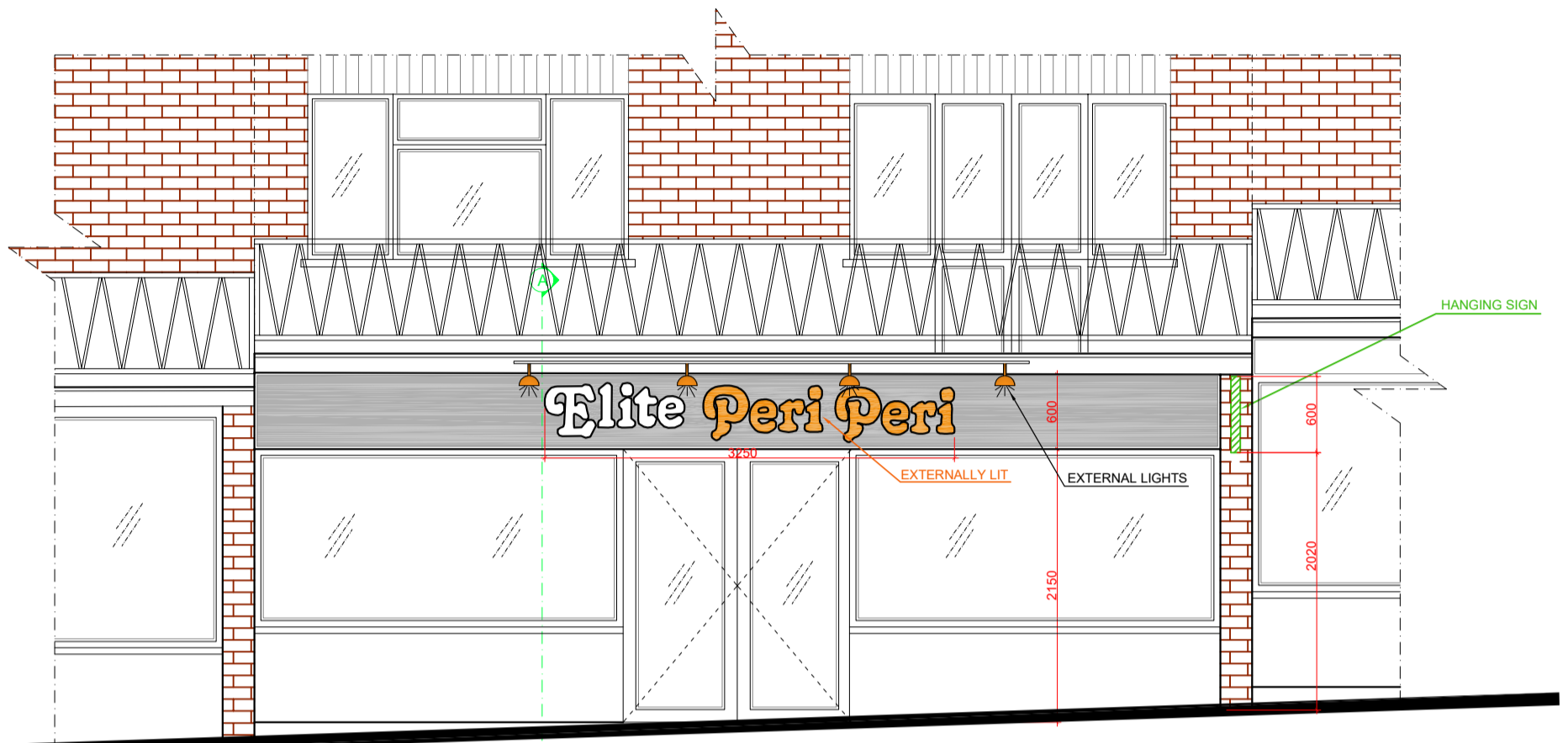
PROPOSED FRONT ELEVATION SCALE: 1/50 @A3
